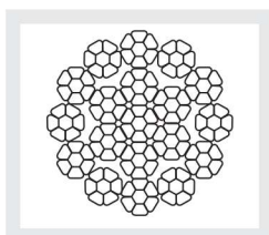
(4) 19 × 7 CMP
